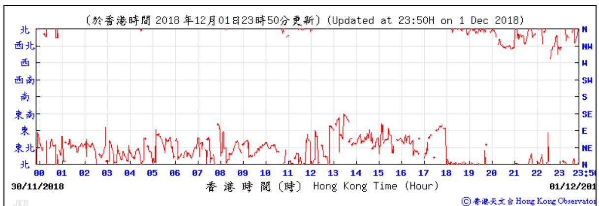
C. Wind Direction extracted from Tseung Kwan O HKO Automatic Weather Station
